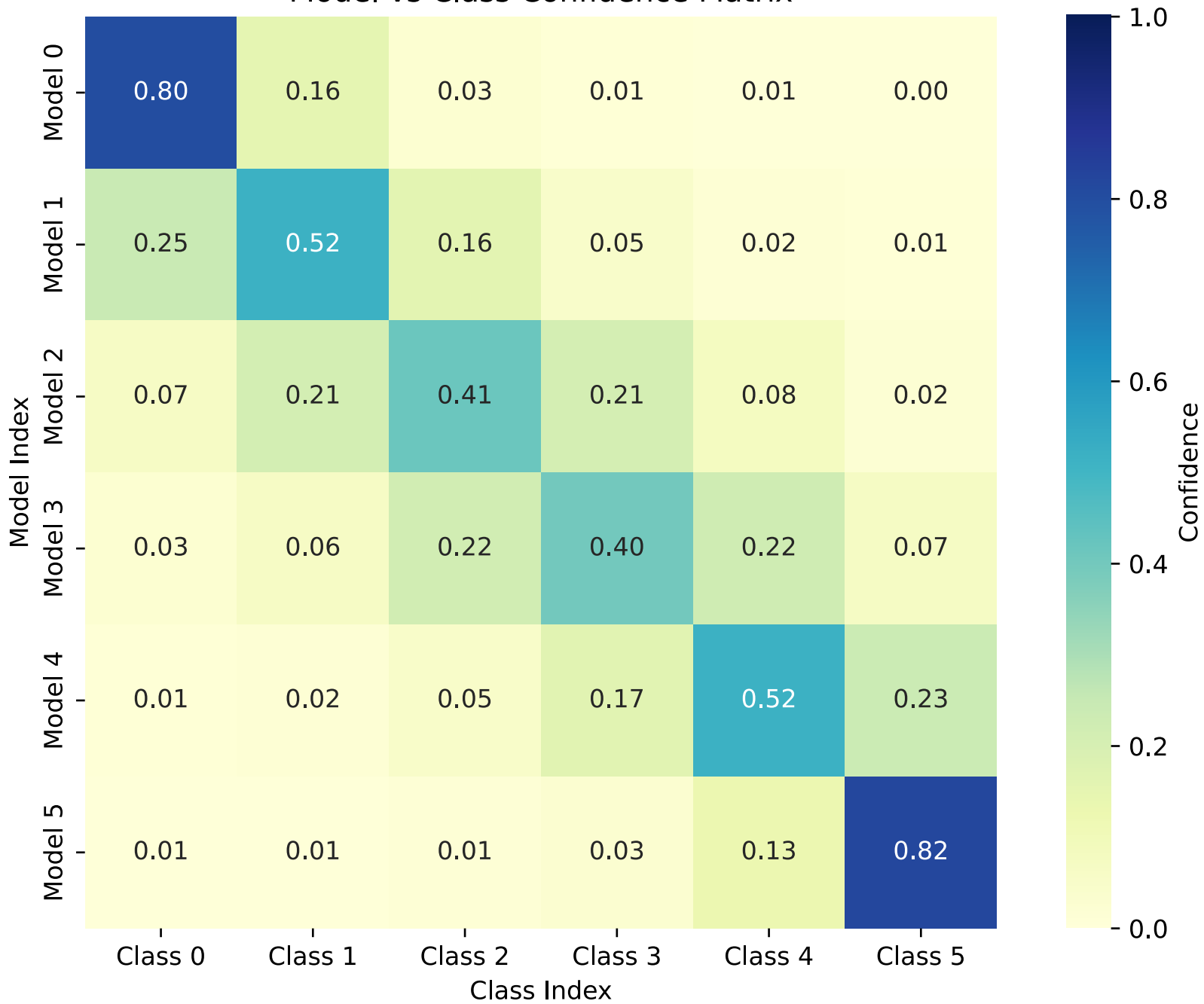
Model vs Class Confidence Matrix
