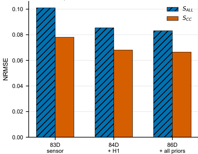
(a) Source-prior ablation
