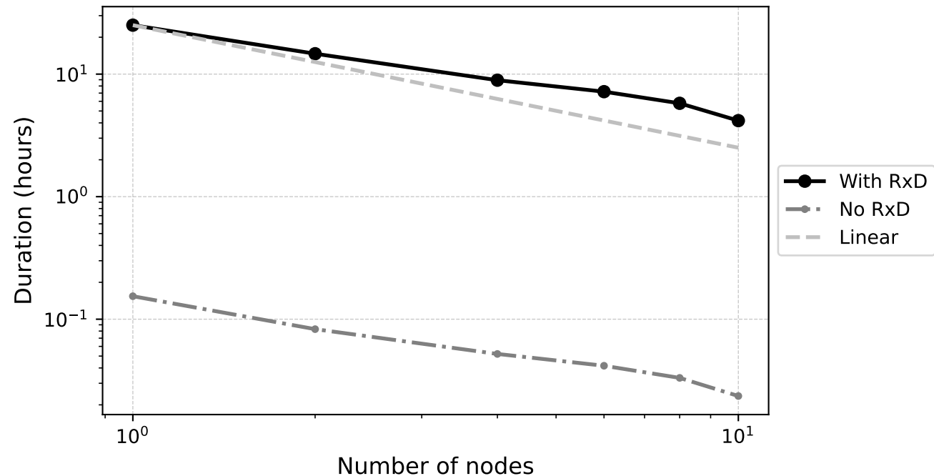
Simulation of 1000 dSPN on HPE Cray EX supercomputer
