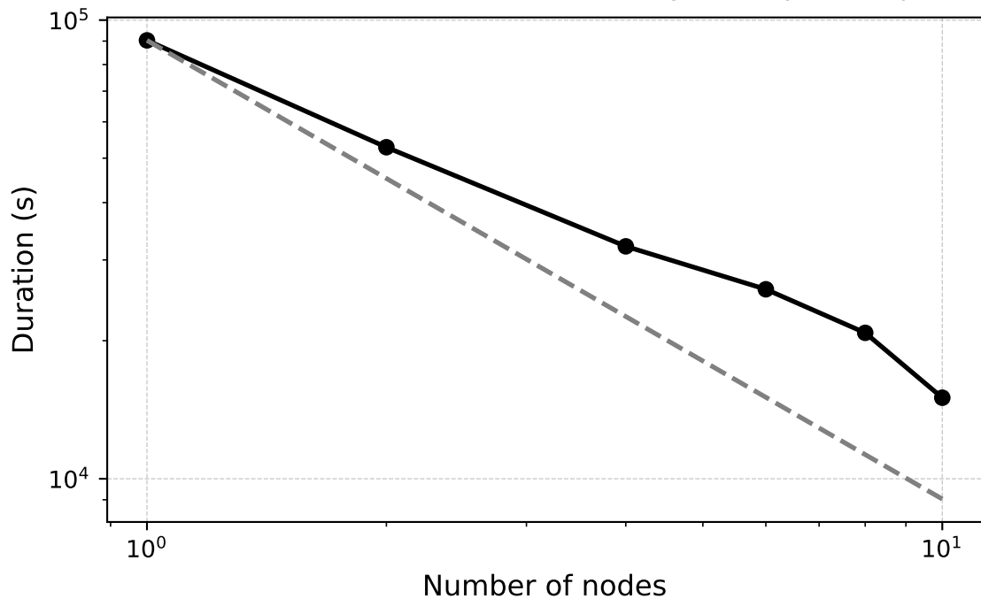
Simulation of 1000 dSPN on HPE Cray EX supercomputer
