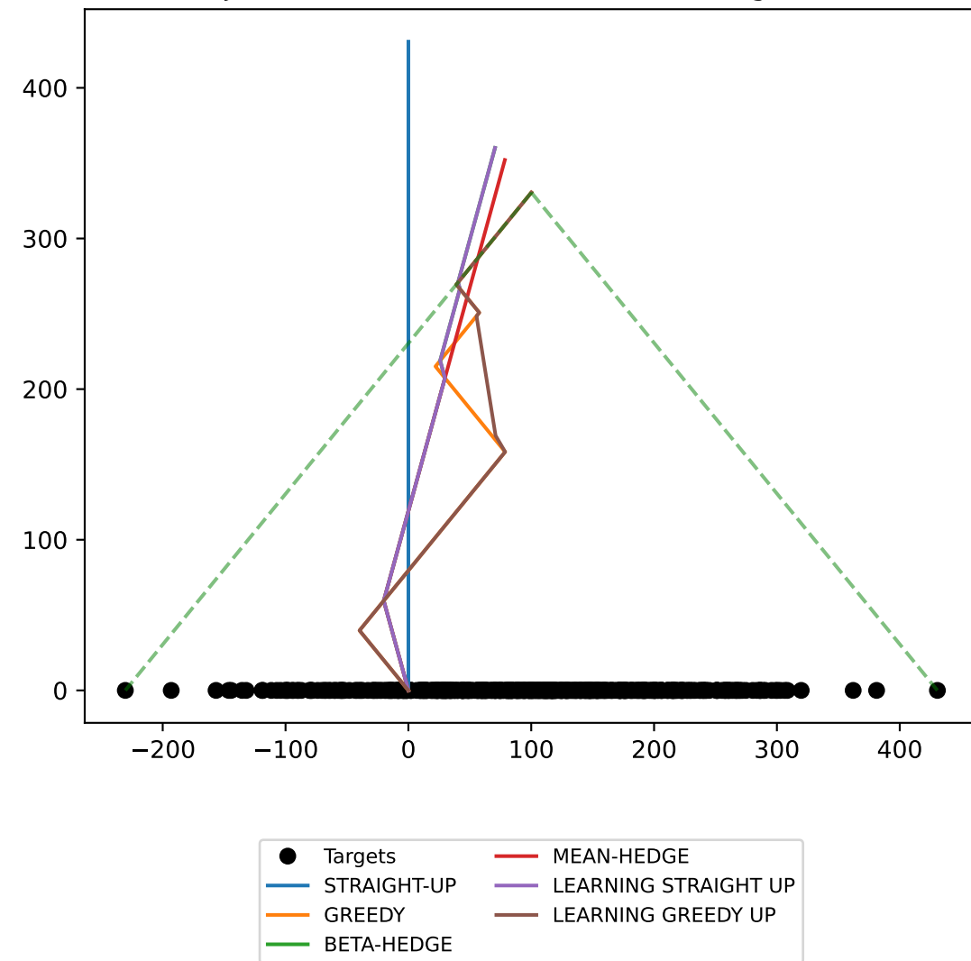
trajectories of the drone for different algorithms
