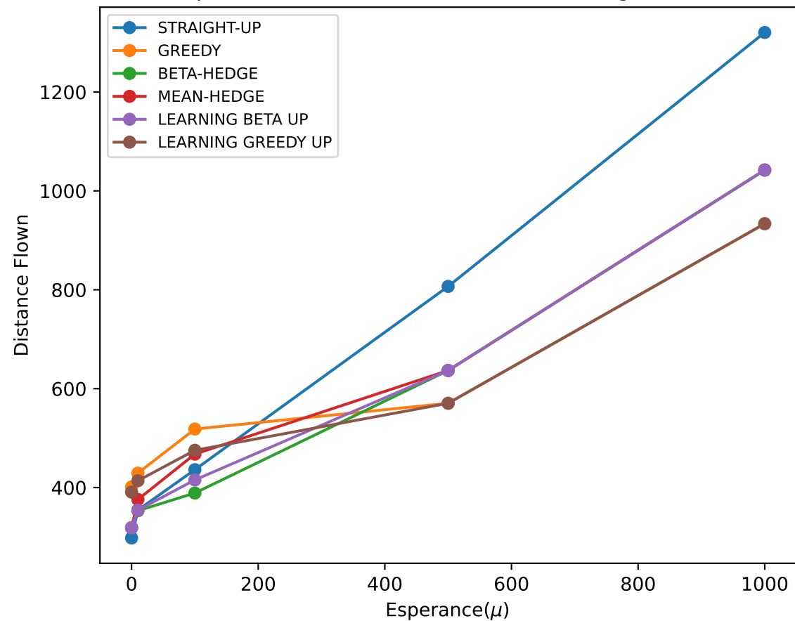
dependence of mu on distance flown, sigma=100
