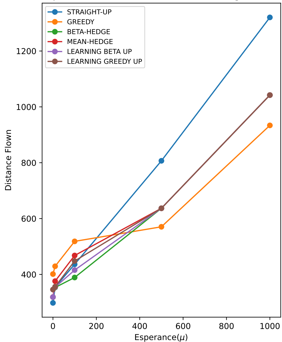
dependence of mu on distance flown, sigma=100
