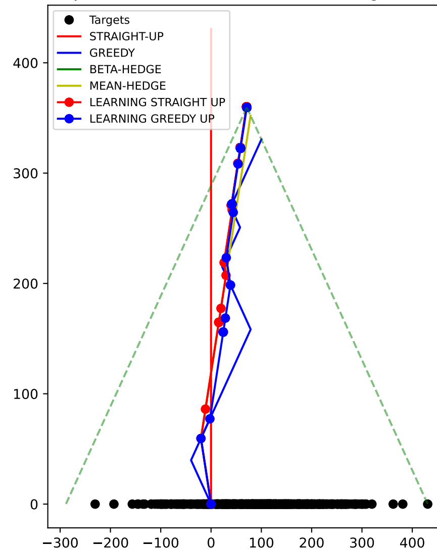
trajectories of the drone for different algorithms
