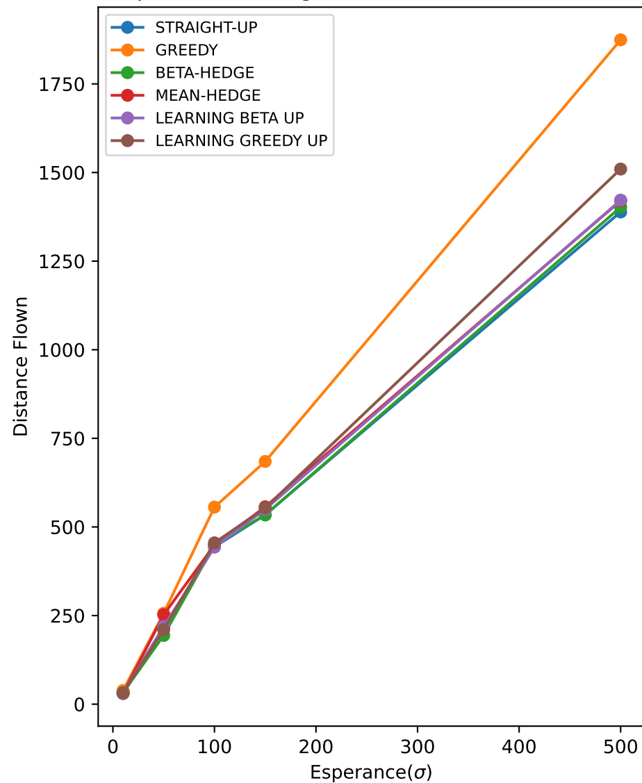
dependence of sigma on distance flown, mu=0
