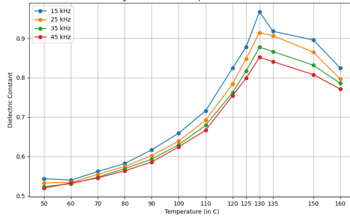
Fig-5: Dielectric Vs Temperature for BaTiO 3
