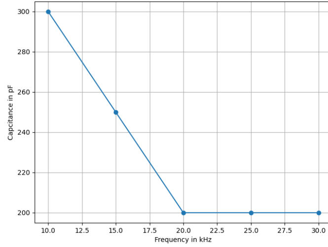
Fig-4: Capacitance Vs Frequency for Disc-Ceramic capacitor
