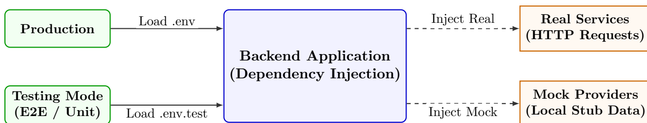
Hình 17: Dependency Injection Mechanism based on Testing Environment
