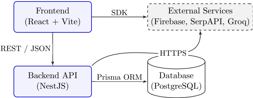
Hình 12: Container Architecture Diagram (C4 Level 2)
