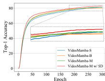
(a) Self-Distillation avoids overfitting.
