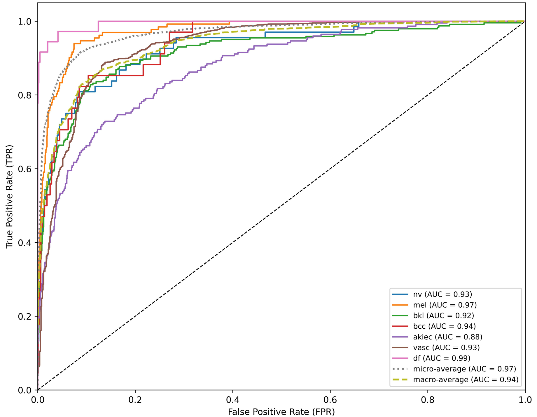
Multi-class ROC curves
