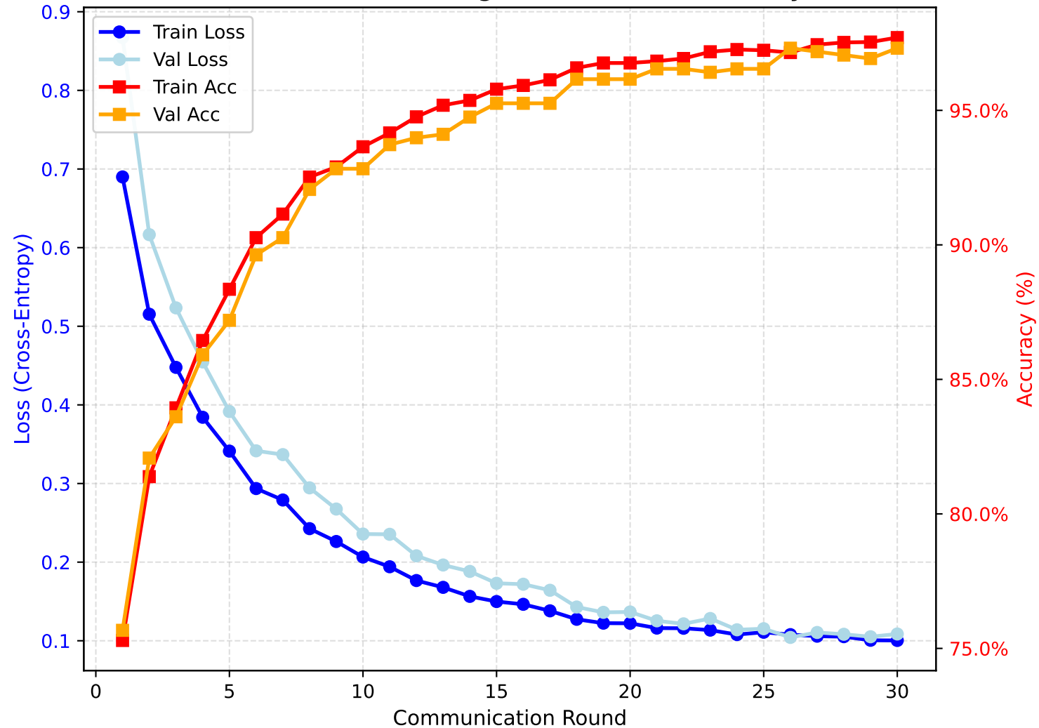
Global Model Convergence: Loss and Accuracy
