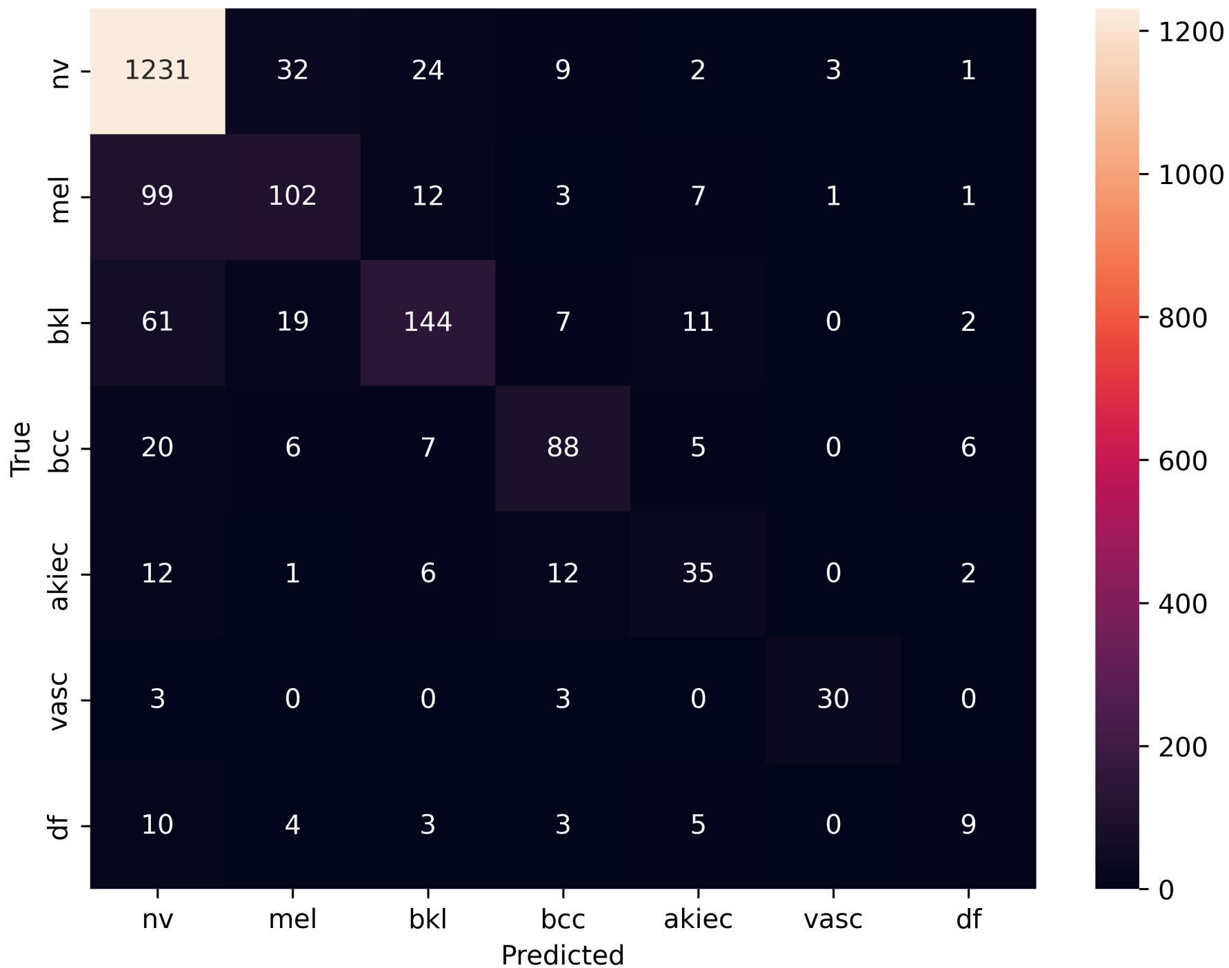
Confusion Matrix (Test set)
