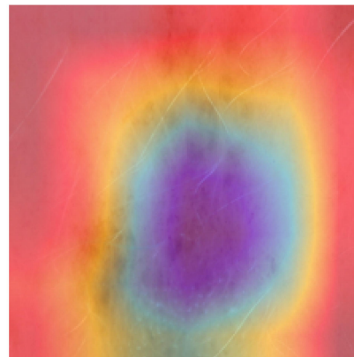
Overlay
