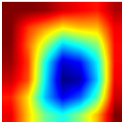
Grad-CAM++ Heatmap
