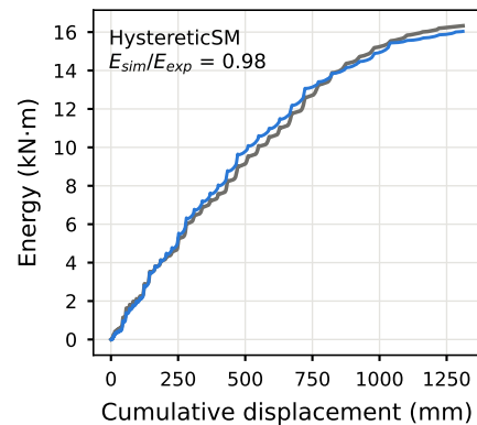
Dissipated energy
