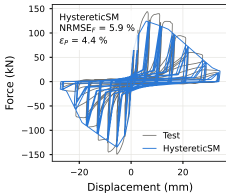
Hysteresis
