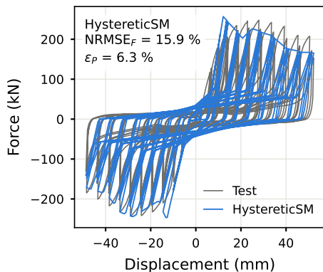
Hysteresis
