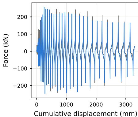
Force history
