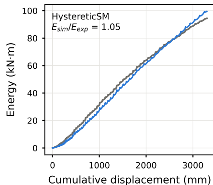
Dissipated energy
