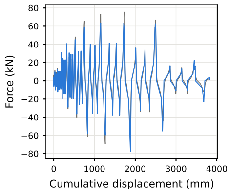
Force history
