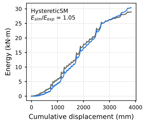
Dissipated energy
