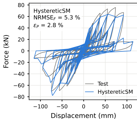
Hysteresis
