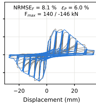
Backbone / peaks (0.5, 3)
