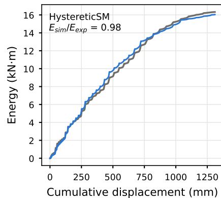
Dissipated energy
