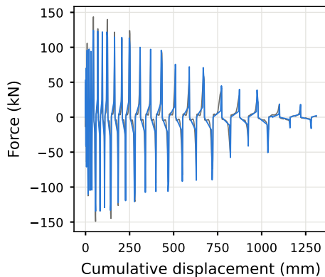
Force history
