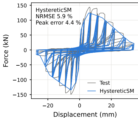
Hysteresis
