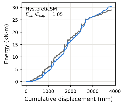
Dissipated energy
