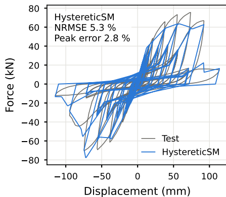
Hysteresis
