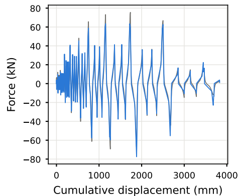
Force history
