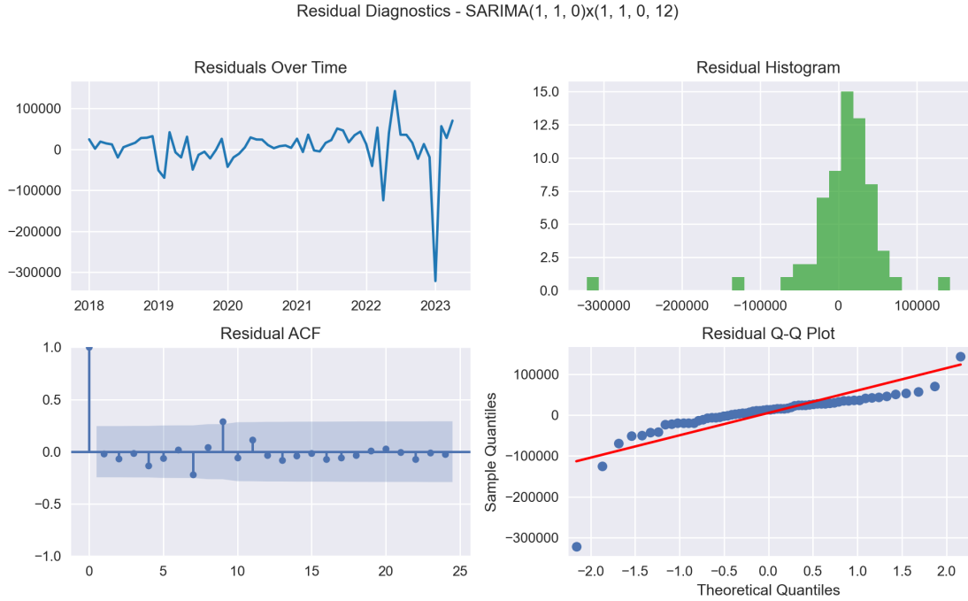
Figure 5: Residual diagnostics for \text{SARIMA}(1, 1, 0) \times (1, 1, 0)_{12} : residuals over time (top left), histogram (top right), residual ACF (bottom left), and Q-Q plot (bottom right). Most autocorrelations lie within the 95% confidence band, and the Ljung-Box p -value at lag 12 is 0.3355, confirming white-noise residuals.
