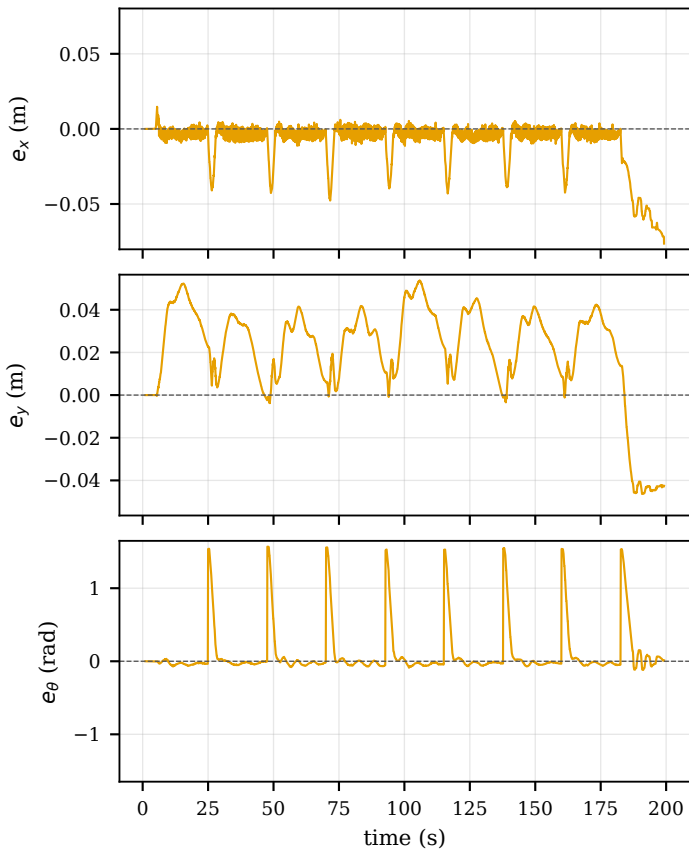
Nominal Backstepping
