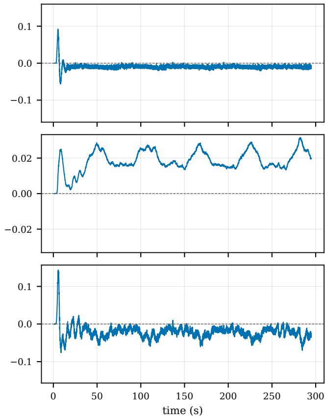
Compensated BSMC
