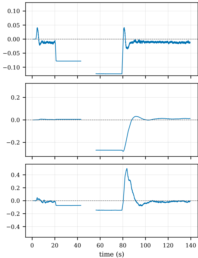
Compensated BSMC
