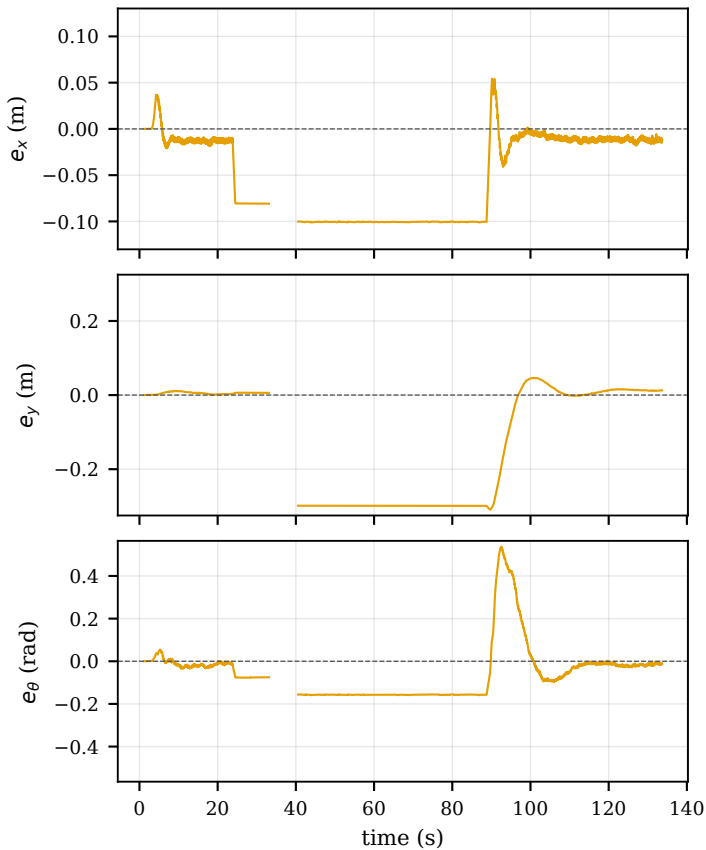
Nominal Backstepping
