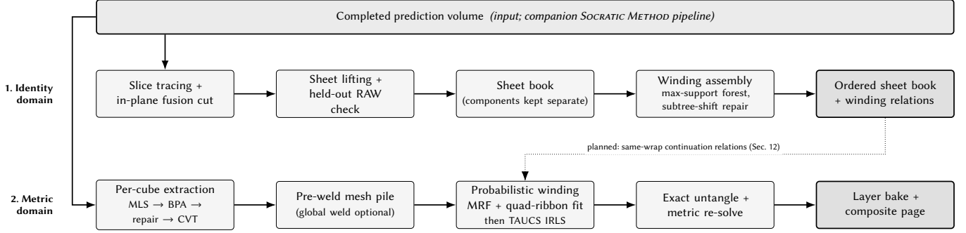
Fig. 2. The ScrollFiesta data flow. Solid arrows carry geometry and volumes; the dotted arrow is a link that does not yet exist. The completed prediction volume is an input rather than a stage: it is produced by the companion Socratic Method pipeline and is never written back to from here. The identity domain decides what is one sheet without fusing geometry. In the metric lane, generalized winding and local relations become uncertain factors in an integer MRF before metric fitting. Both lanes read the same volume independently, which is what makes a change to that volume measurable through either one in isolation.
