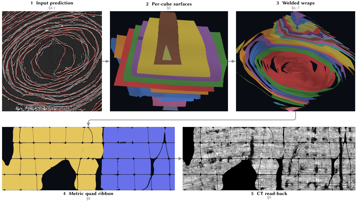
Fig. 1. ScrollFiesta end to end, on one PHerc0139 4 \times 5 \times 5 block. (1) The input: a completed coarse surface prediction (red) over raw CT at z=4416 . Producing that volume without inventing a connection onto a neighbouring turn is the subject of the companion Socratic Method report; ScrollFiesta takes it as given (Section 4.1). (2) One 128^3 cube after moving-least-squares collapse, guarded ball pivoting, and topological cleanup, with each extracted sheet coloured separately. The sheets stay distinct components, so no two wraps in this cube are fused into one surface. (3) The welded block seen down the scroll axis. Welding joins fronts across cube seams only where both cubes agree on the wrap, so the wraps survive as long, separately identified spirals rather than one merged surface. (4) A window of the solved flat atlas, coloured by atlas group and cut into metric quad cells. (5) The same window of the CT read-back — the papyrus those exact cells carry. Black is absent material rather than missing texture: no layer supplies papyrus there, and the pipeline leaves the hole visible rather than interpolating across it. Figure 2 gives the same pipeline as a data-flow diagram.
