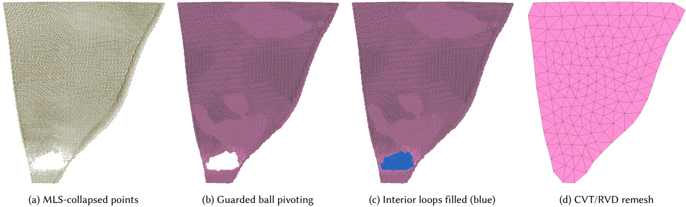
Fig. 3. The per-cube extraction stages on one PHerc0139 sheet. (a) Voxel-centre points after the iterated MLS projection has collapsed the several-voxel-thick prediction to a single sheet. (b) The consistently oriented, guarded ball-pivoting reconstruction; the remaining perforations are prediction gaps, not meshing failures. (c) Clean interior loops are closed (filled regions in blue) while the genuine sheet boundary is left open. (d) The level-of-detail stage on the same sheet: the CVT/RVD remeshing of Section 5.5 relocates samples into a near-isotropic blue-noise distribution.
