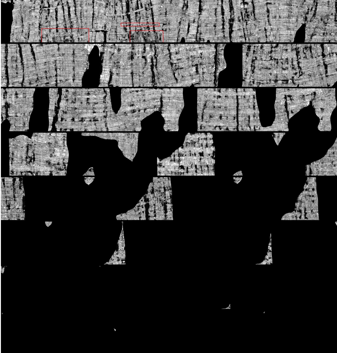
Fig. 7. The 4 \times 5 \times 5 fixed-topology metric composite, reformatted from its native 31,127 \times 508 ribbon into reading rows. All 4,033,291 faces are conserved. Red boxes mark the previously identified dropout sites; evidenced secondary layers now cover them. Black areas remain unsupported rather than being presented as papyrus.
