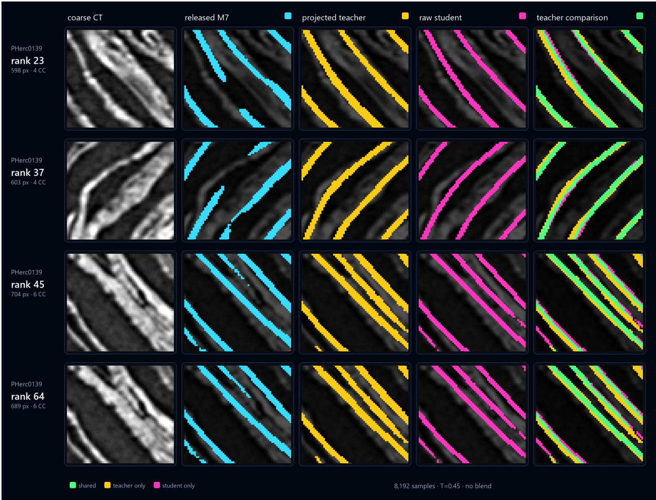
Fig. 5. Locked PHerc0139 comparisons at the selected operating point. Columns show the same CT crop, released M7, projected fine-teacher target, raw student, and a two-sided teacher comparison. Green denotes shared foreground, yellow teacher-only foreground, and magenta student-only foreground.
