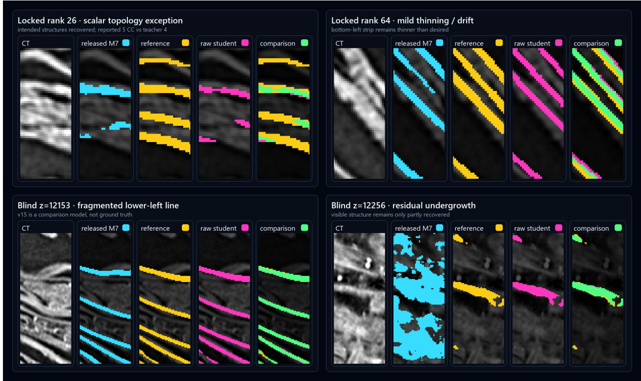
Fig. 6. Known edge cases at t = 0.45 : a component-count proxy that disagrees with the visible structure, mild drift or thinning on locked sheets, and blind PHerc1447 views that remain undergrown or fragmented. Every row includes CT, released M7, the available model-derived reference, raw M7-XR, and a two-sided comparison. Yellow reference masks are not ground truth.
