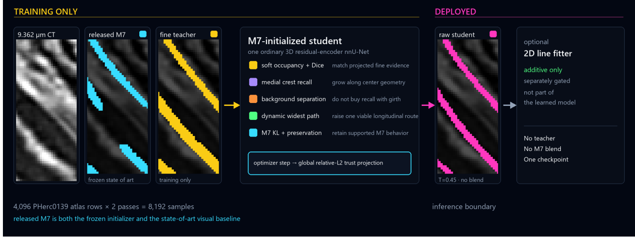
Fig. 2. Method overview with a registered crop. The released M7 appears both as the frozen initializer and as the state-of-the-art visual baseline. Training-only components (fine teacher, projection, medial and separation losses, and post-update trust projection) are separated from the deployed raw student. The optional 2D fitter is outside the learned model and is evaluated separately.
