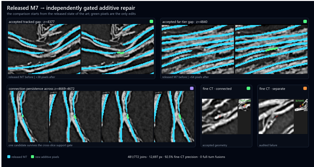
Fig. 4. Measured line-fitter behavior on the released M7 baseline. Left: representative M7 masks before and after additive accepted joins. Center: the same connection persists across neighboring z-slices. Right: registered fine-CT evidence distinguishes a supported connection from a required separation. The calibration accepted 481 of 772 proposals, added 12,697 pixels, reached 92.5% registered fine-CT precision, and produced no observed full-turn fusion. Cyan is released M7 and green is fitted addition.
