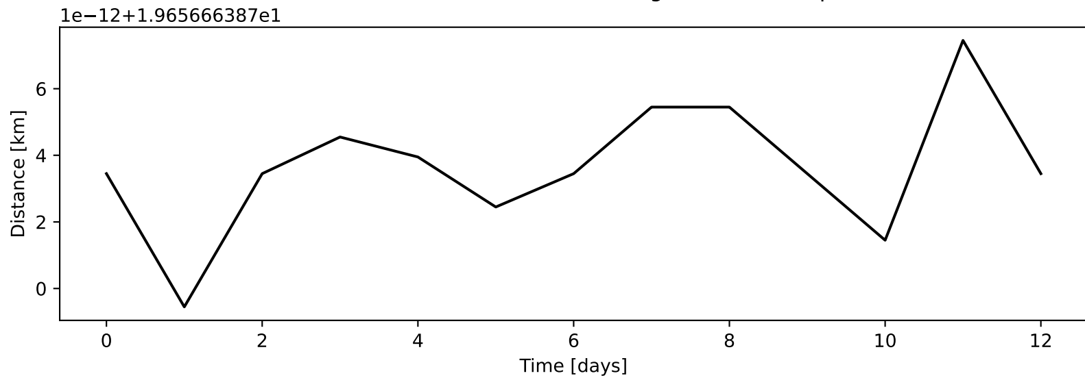
Great-circle distance between MITgcm and exact peak
