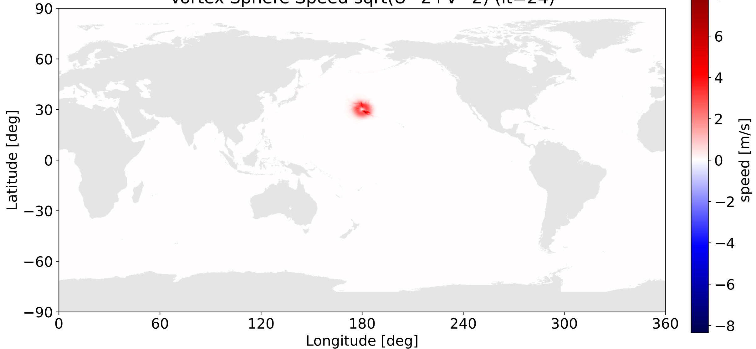
Vortex Sphere Speed \sqrt{U^2+V^2} (it=24)
