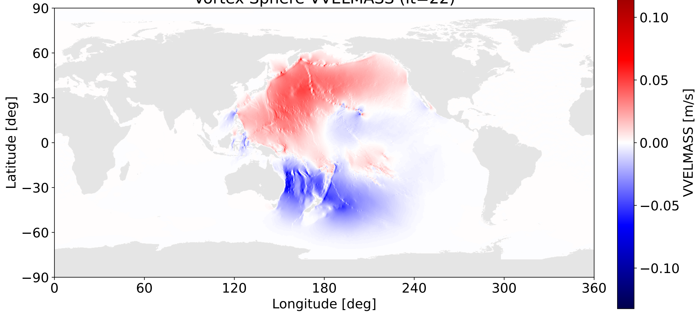
Vortex Sphere VVELMASS (it=22)
