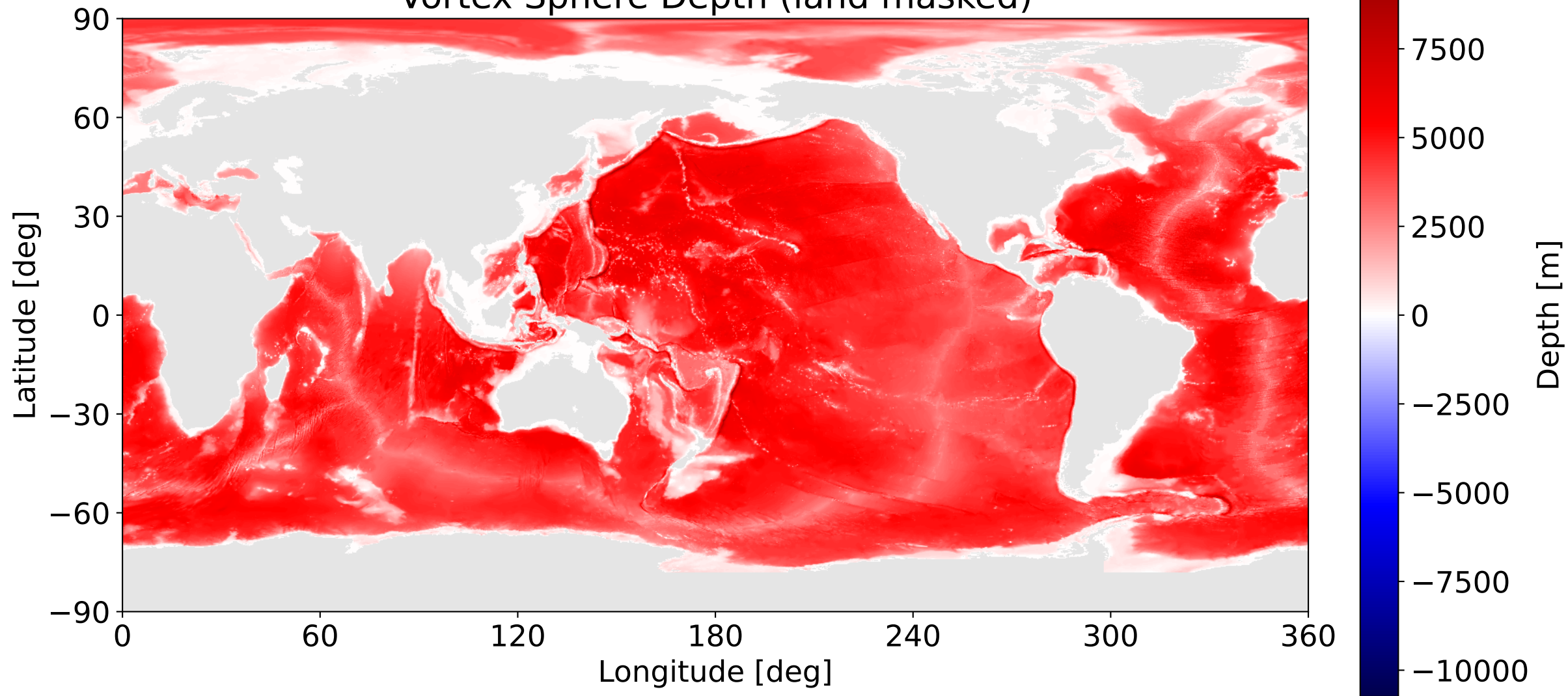
Vortex Sphere Depth (land masked)
