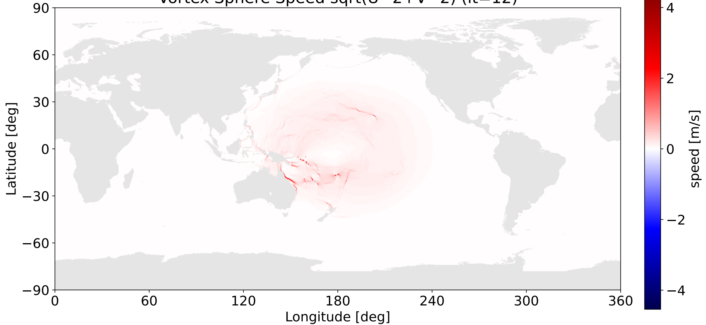
Vortex Sphere Speed \sqrt{U^2+V^2} (it=12)
