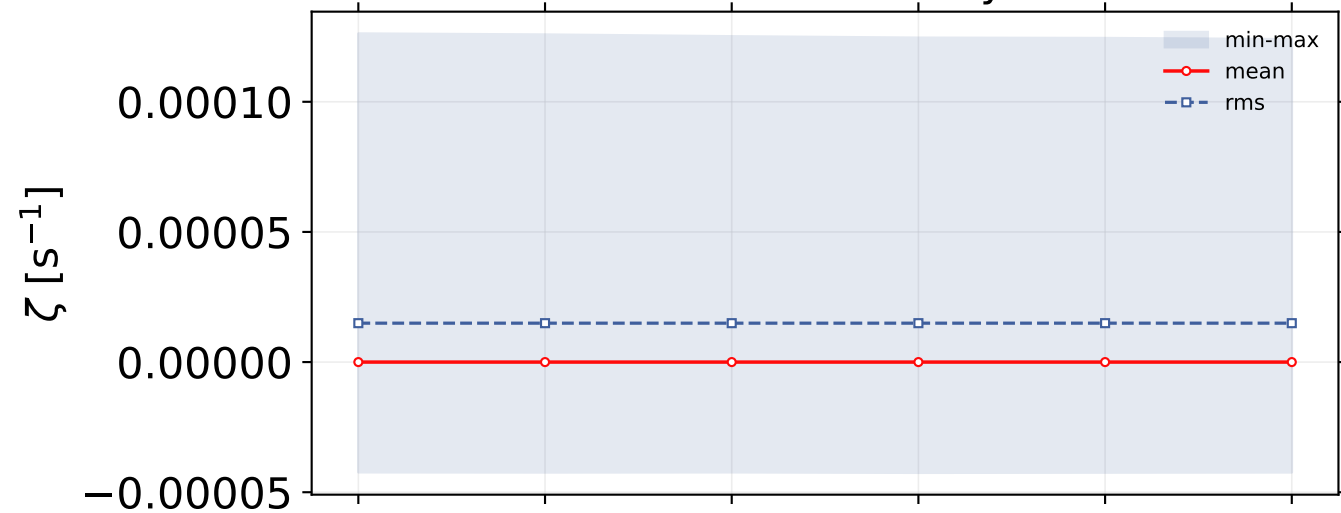
Relative vorticity
