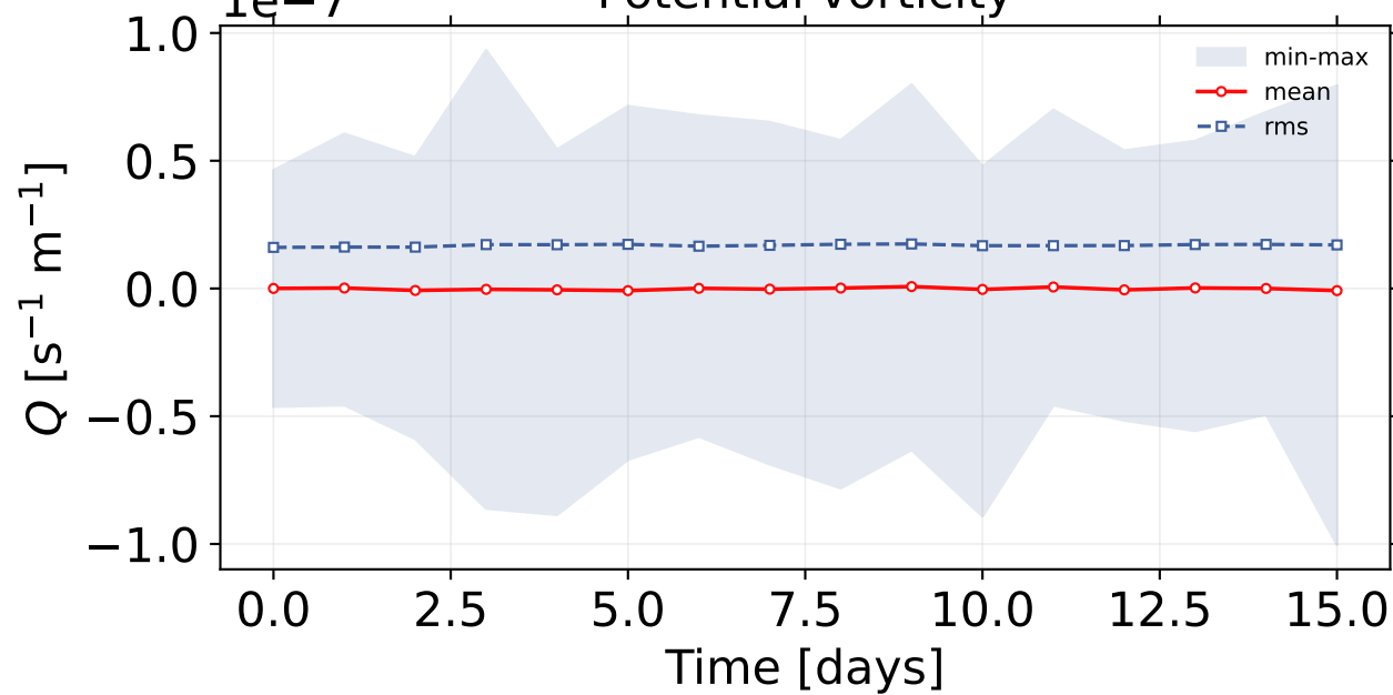
Potential vorticity
