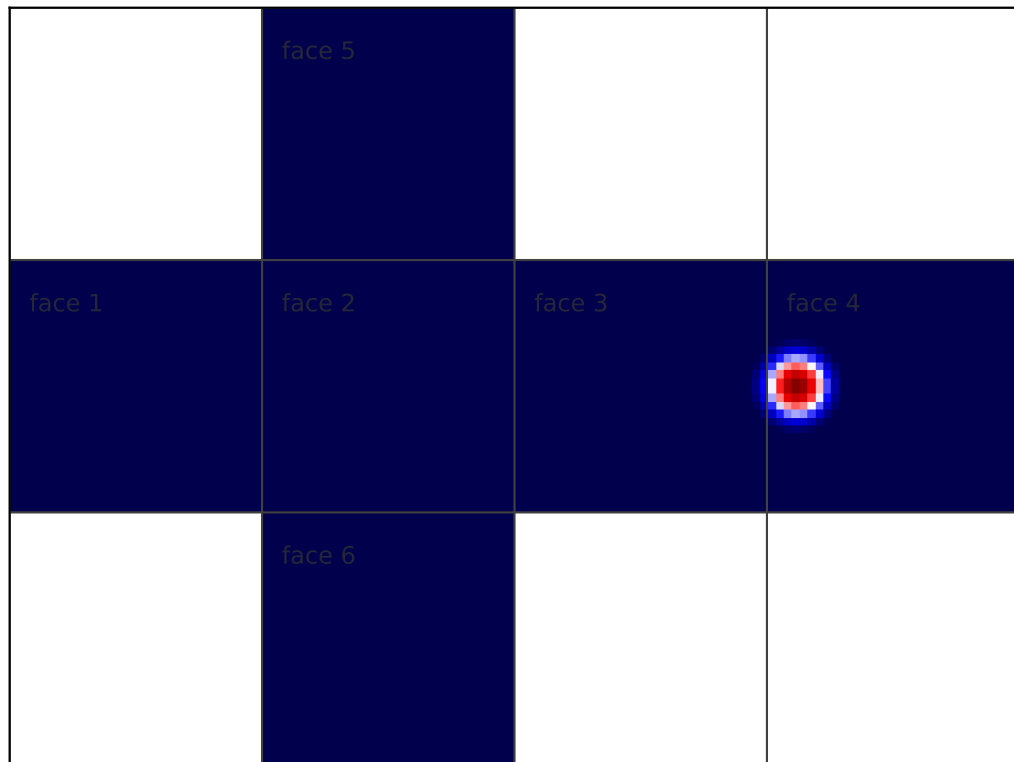
advect_cs final exact tracer | alpha=0
