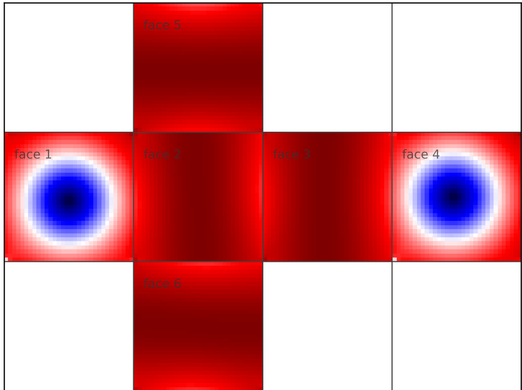
advect_cs velocity magnitude | alpha=1.52
