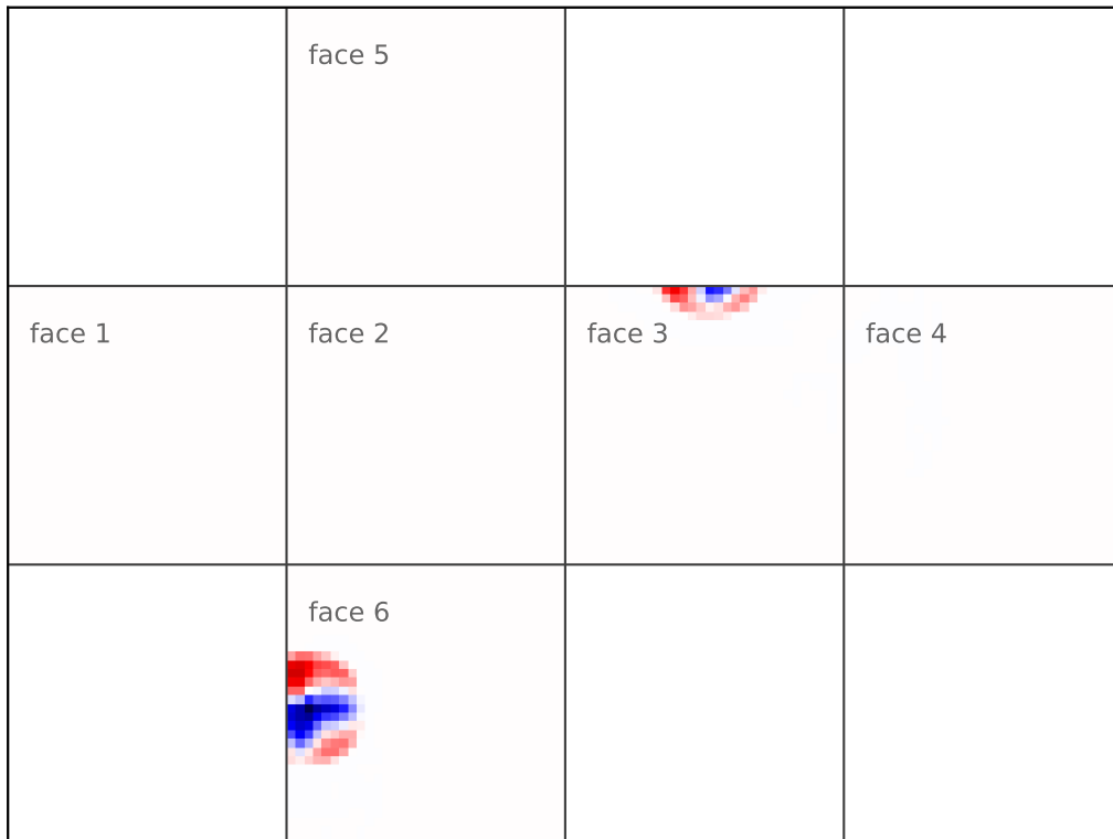
advect_cs S error | alpha=0.05 | day=3.00
