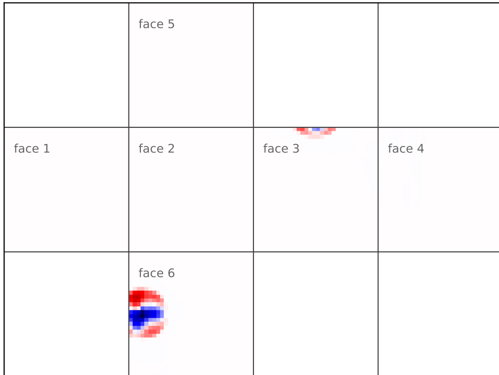
advect_cs S error | alpha=0 | day=3.00
