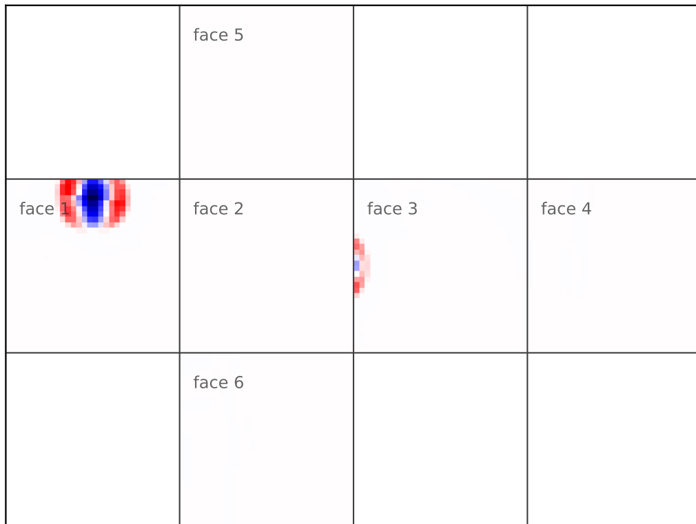
advect_cs S error | alpha=0 | day=6.00
