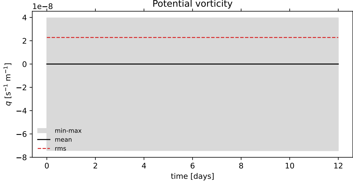
Potential vorticity
