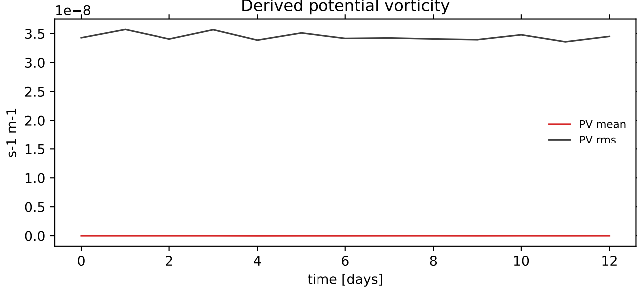
Derived potential vorticity
