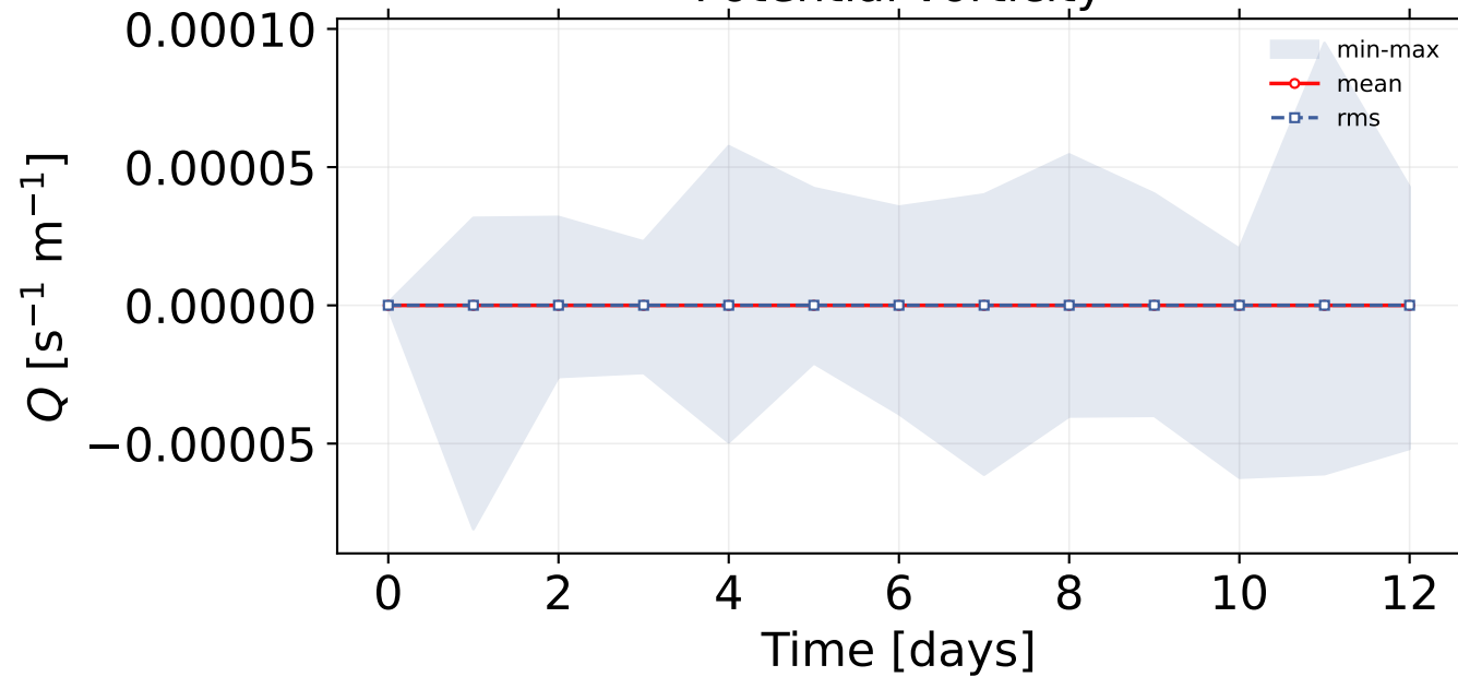
Potential vorticity
