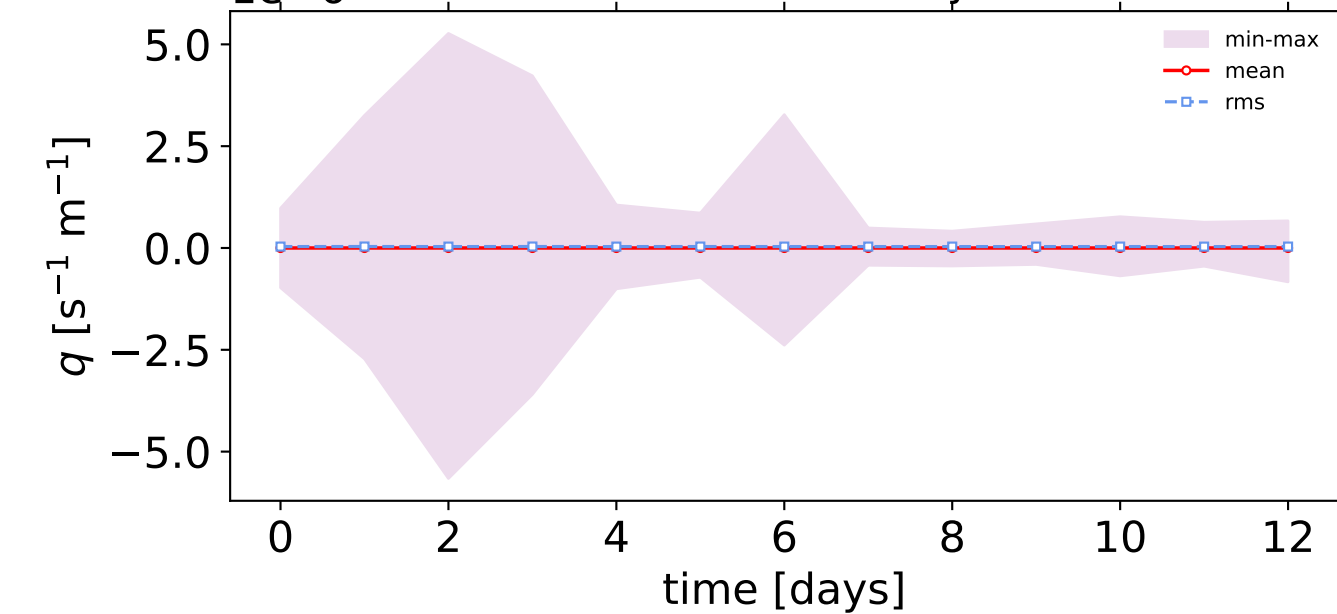
Potential vorticity
