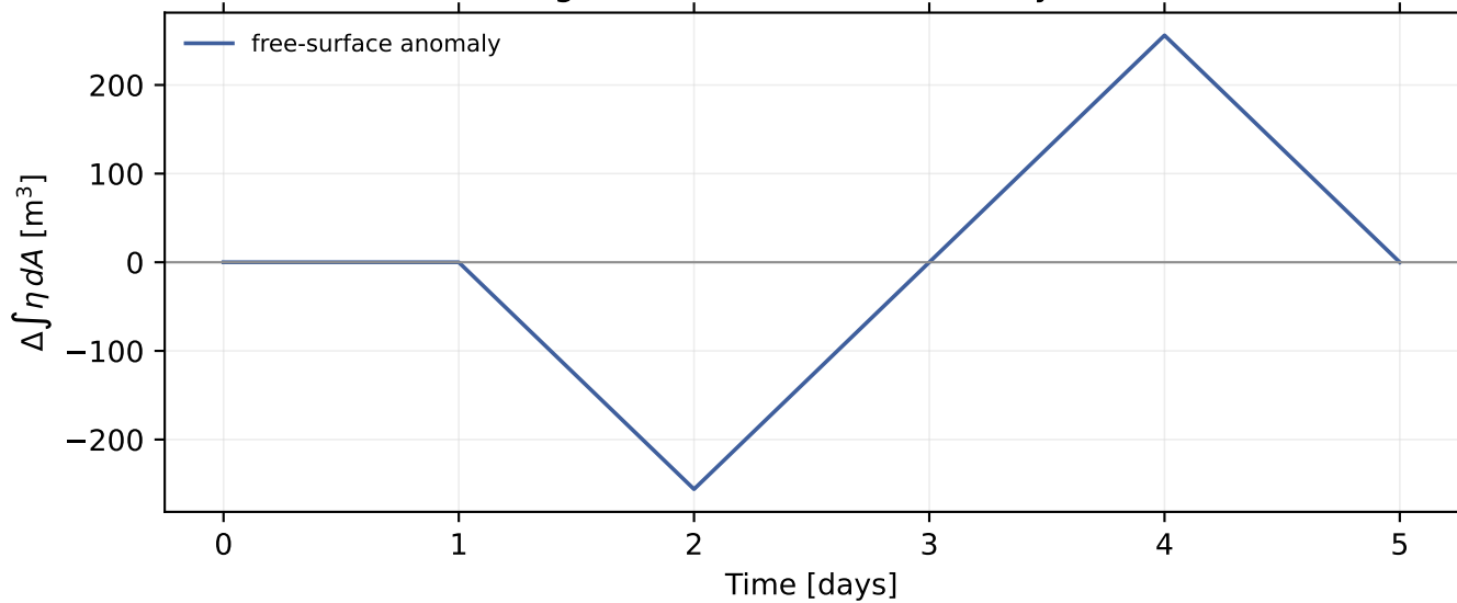
Integrated free-surface anomaly drift
