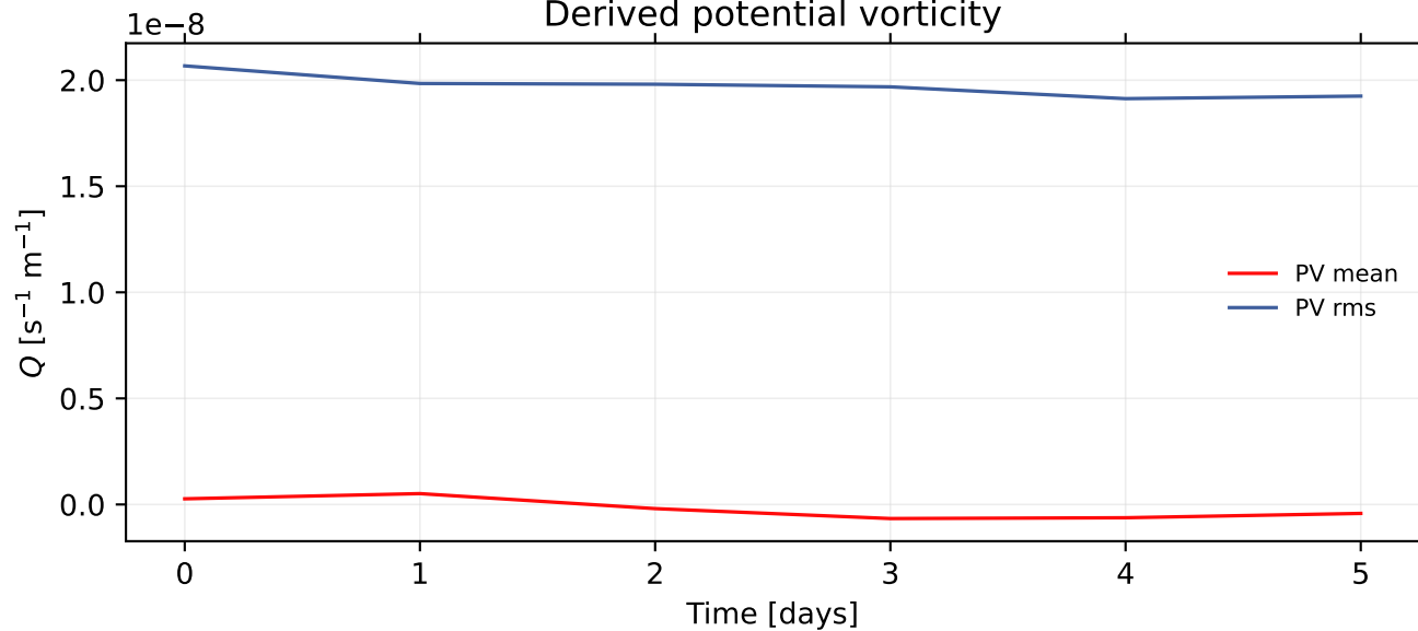
Derived potential vorticity
