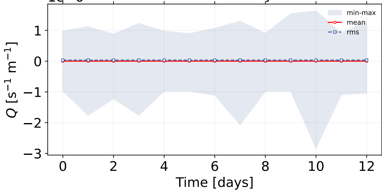
Potential vorticity
