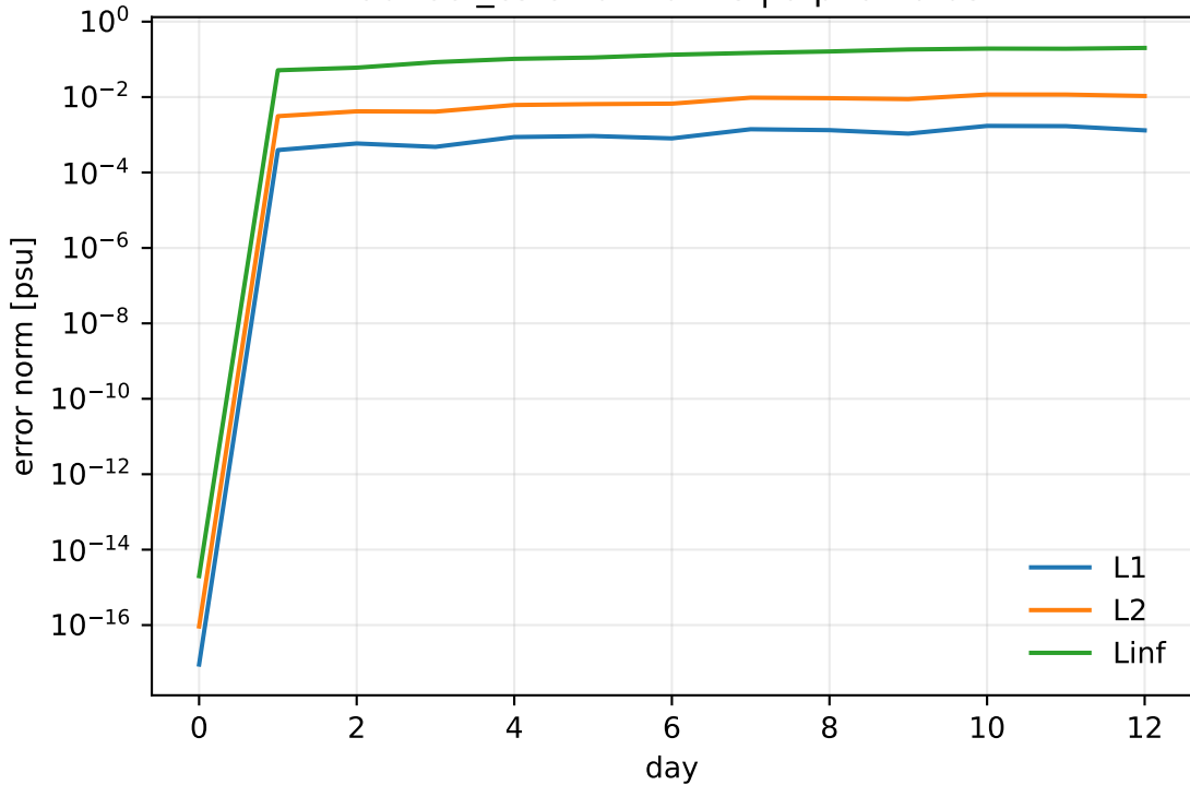
advect_cs error norms | alpha=0.05
