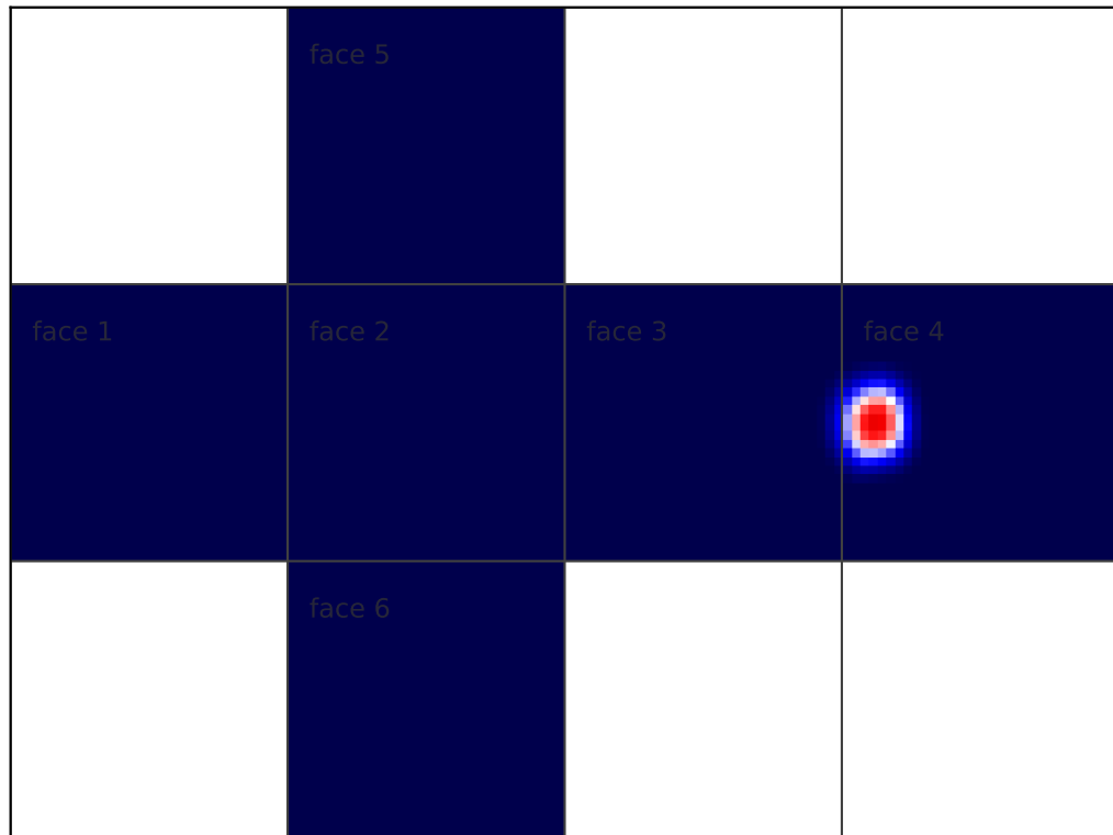
advect_cs final model tracer | \alpha=0.05
