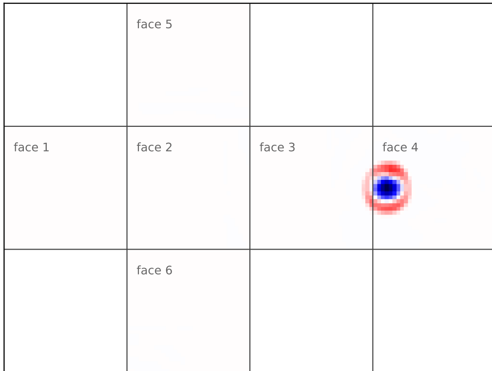
advect_cs final tracer error | alpha=1.52
