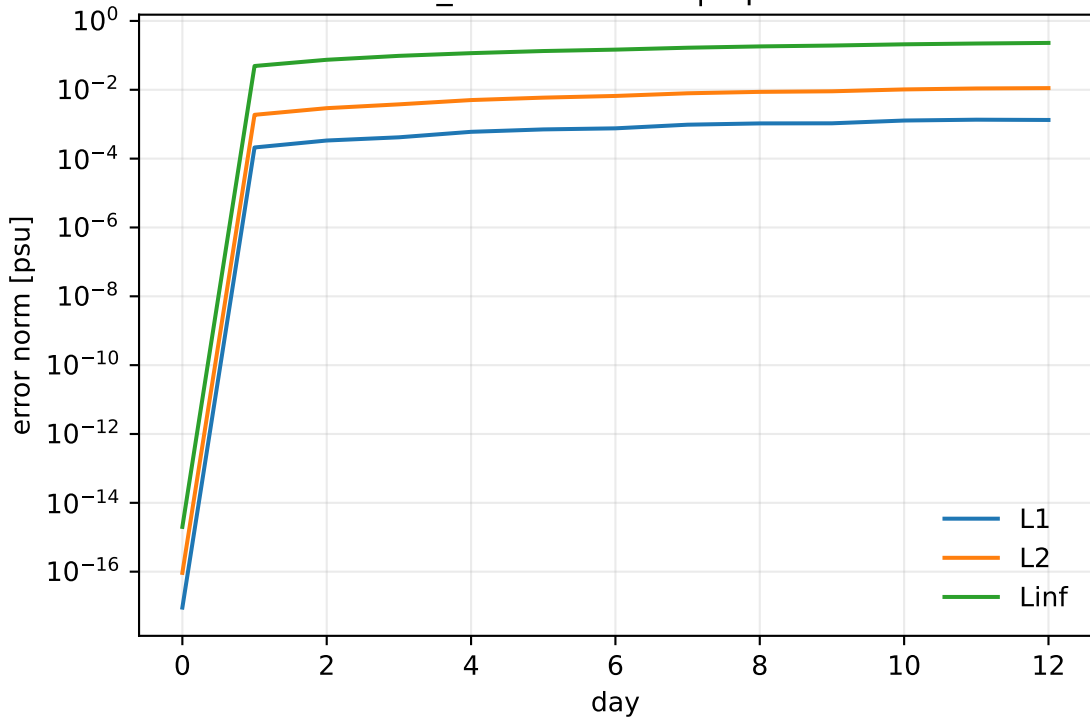
advect_cs error norms | alpha=1.57
