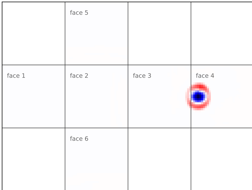
advect_cs final tracer error | alpha=1.57
