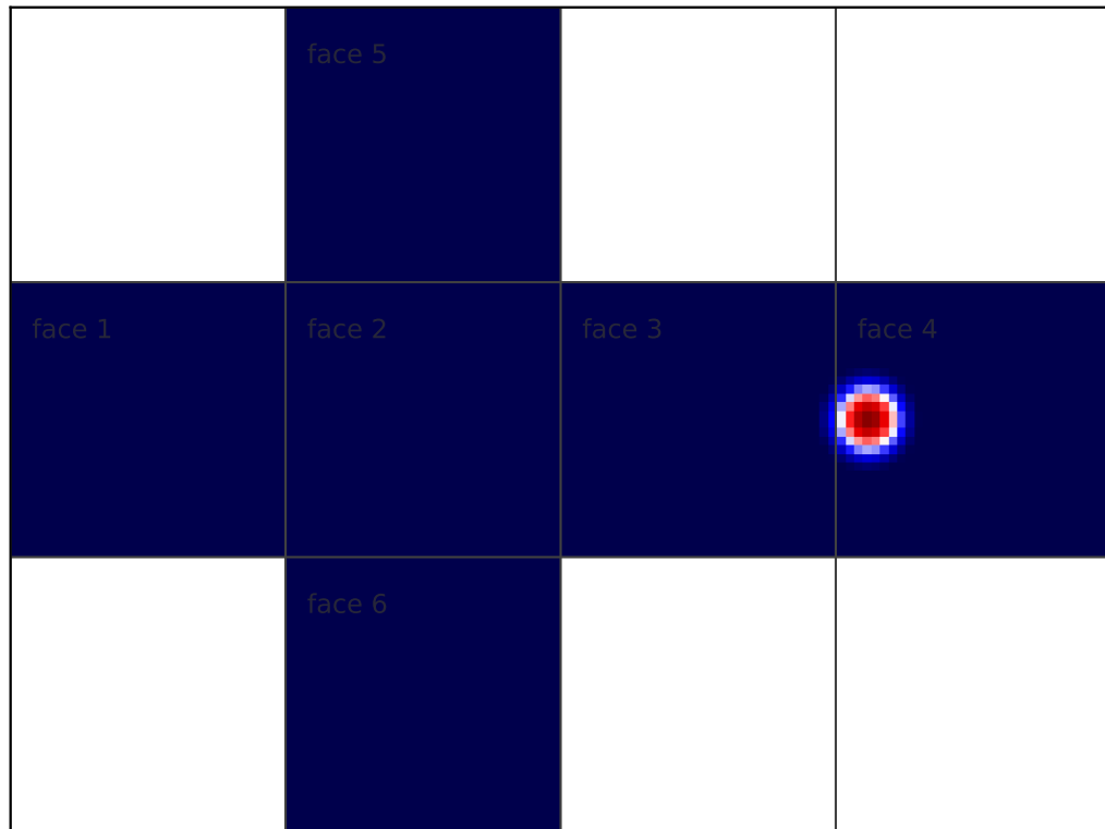
advect_cs final exact tracer | alpha=1.57
