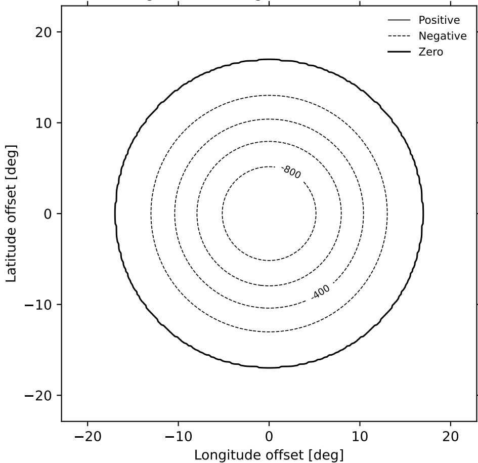
Signed Error - MITgcm (200 m contours)
