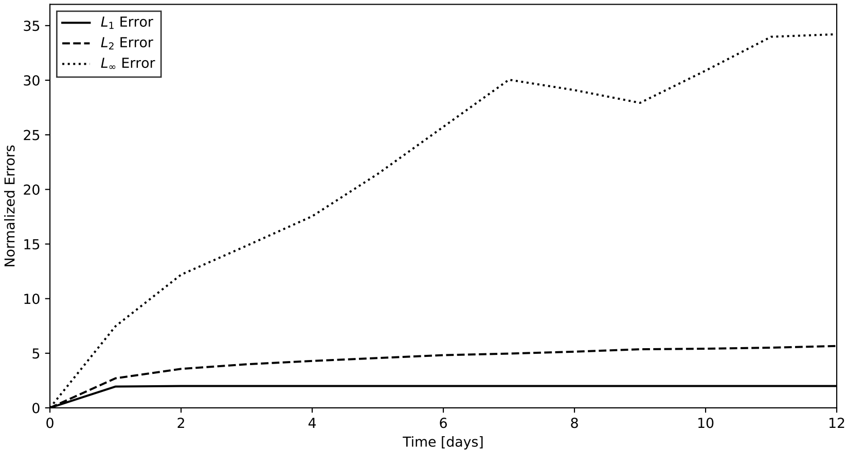
TC1 normalized error growth | Eta moves; check error norms
