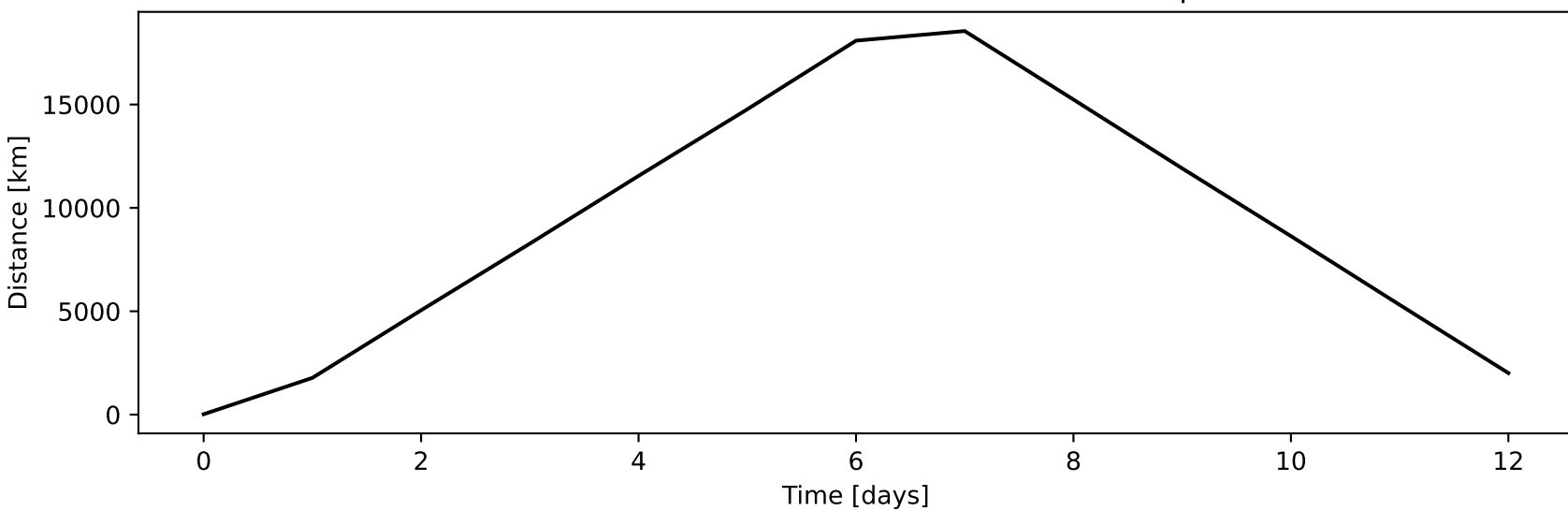
Great-circle distance between model and exact peak
